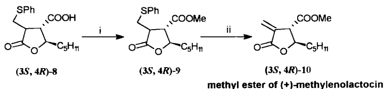
Scheme III Reagents and conditions: i, \text{CH}_2\text{N}_2 , \text{Et}_2\text{O} , rt; ii, a) m -CPBA, \text{CH}_2\text{Cl}_2 , -10^\circ\text{C} ; b) toluene, reflux.
